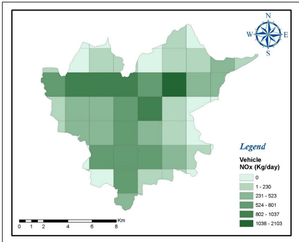
Figure 3.76: Spatial Distribution of NOx Emissions from Vehicles
