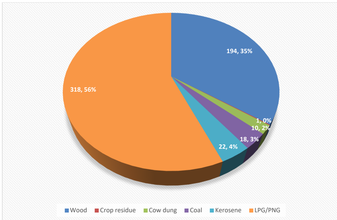
Figure 3.18: NO x Emission load from Domestic Sector (Kg/day, %)
