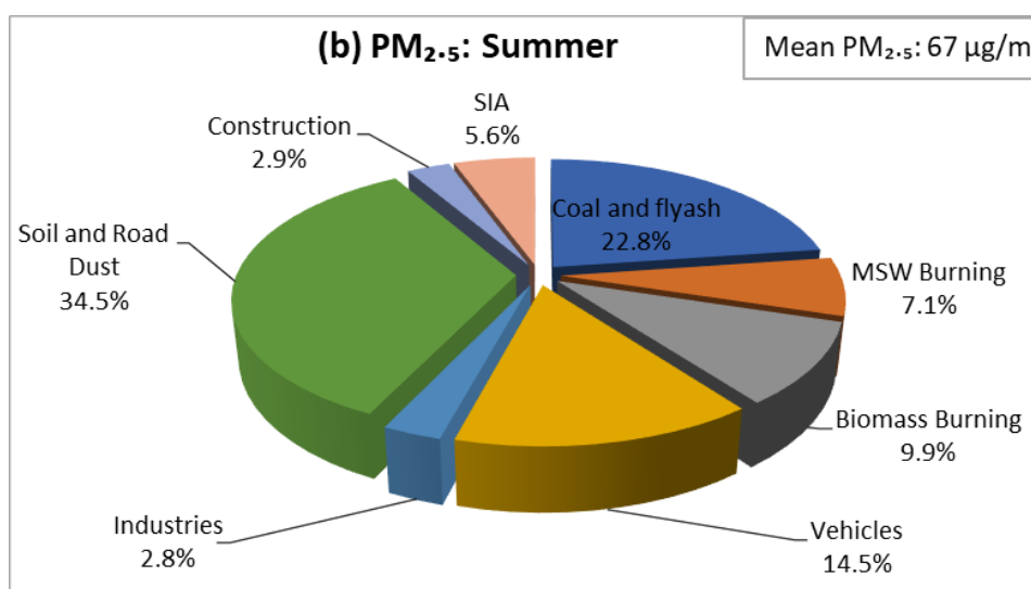
Figure 4.36: Overall source contribution to PM 2.5 in (a) winter and (b) summer
